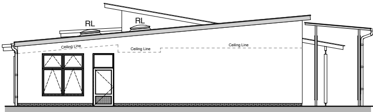
Proposed North Facing Elevation (B)
