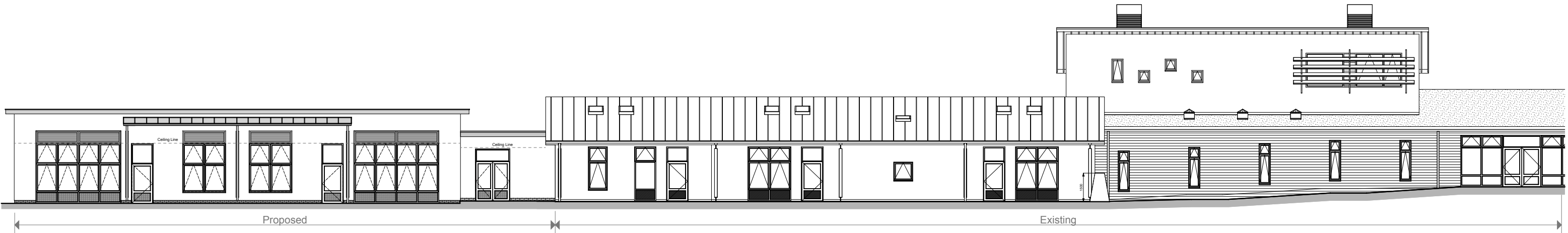
Proposed West Elevation (A)
