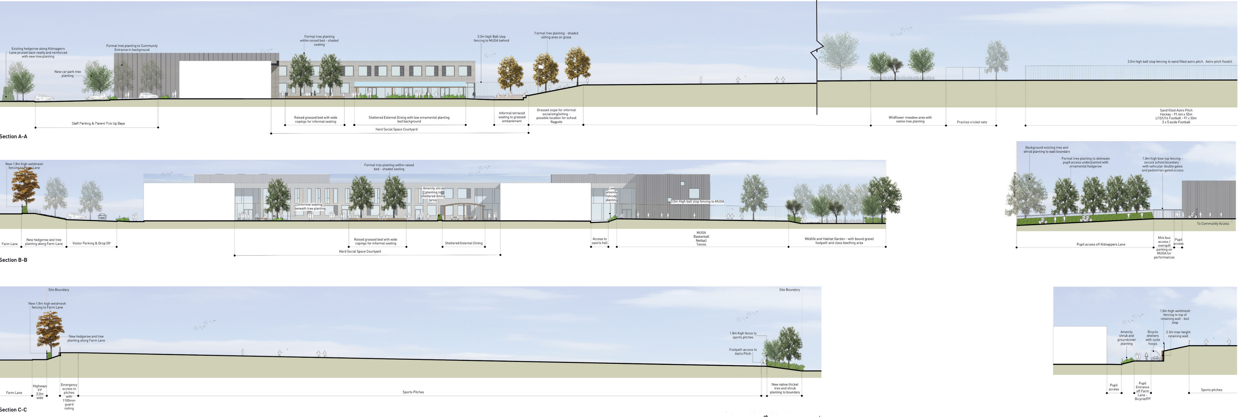
SITE SECTIONS
